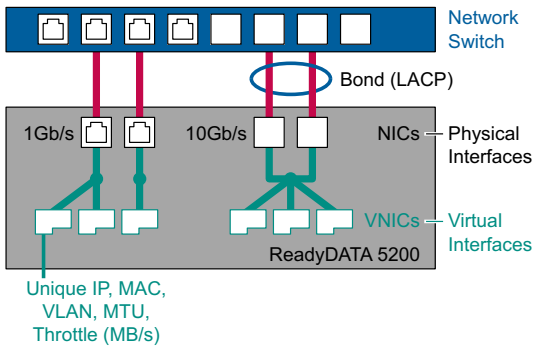
Figure 5. Virtual network interfaces
